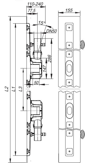
douchegoot CeraLine F Duo 800 – 1200
