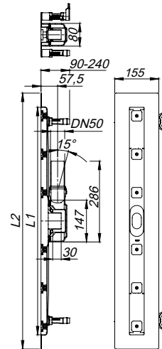
douchegoot CeraLine Plan F 500 – 1200
