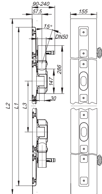
douchegoot CeraLine Plan F Duo 800 – 1200
