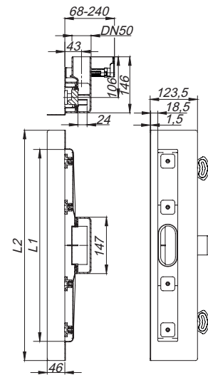
douchegoot CeraLine Nano W 500 – 1200
