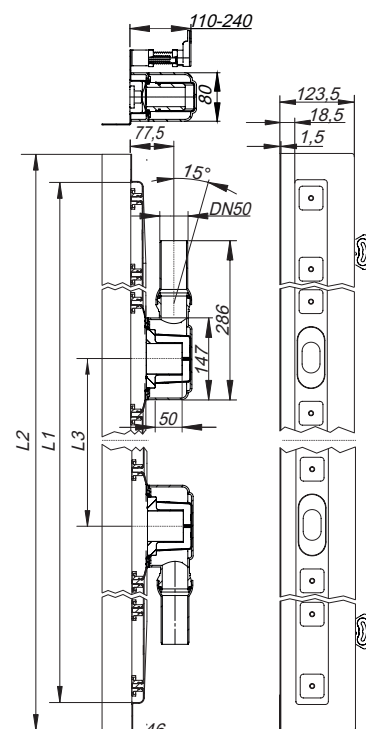
douchegoot CeraLine W Duo 800 – 1200
