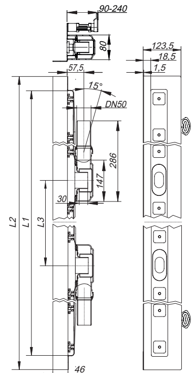
douchegoot CeraLine Plan W Duo 800 - 1200
