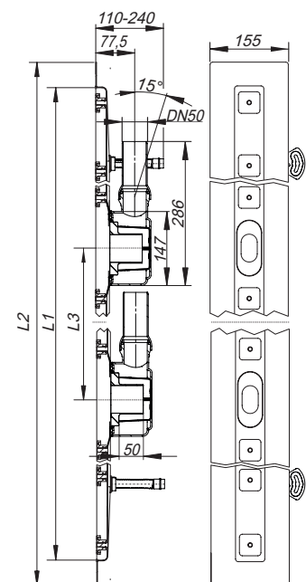
douchegoot CeraLine F Duo 1300 – 2000
