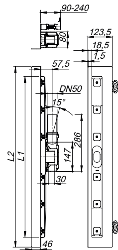
douchegoot CeraLine Plan W 500 – 1200
