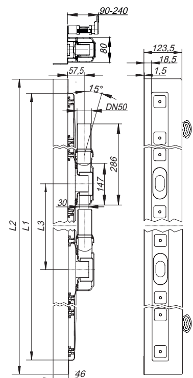
douchegoot CeraLine Plan W Duo 1300 – 2000
