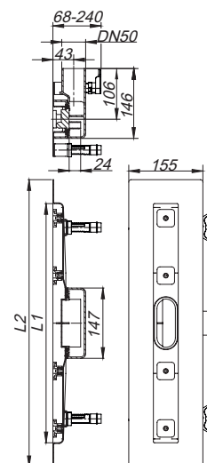
douchegoot CeraLine Nano F 500 – 1200
