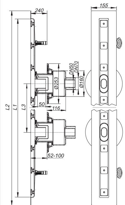
CeraLine verticaal F Duo 1300 – 2000
