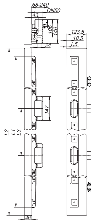
douchegoot CeraLine Nano W Duo 800 – 2000
