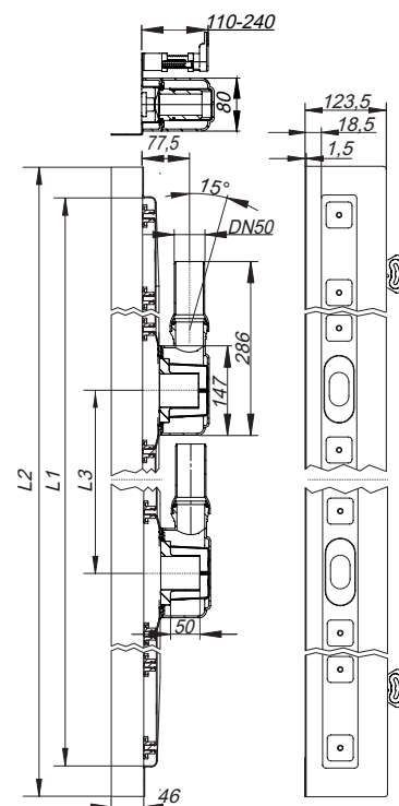
douchegoot CeraLine W Duo 1300 – 2000
