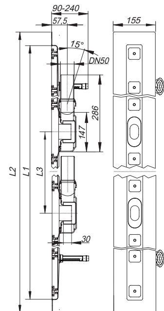
douchegoot CeraLine Plan F Duo 1300 – 2000
